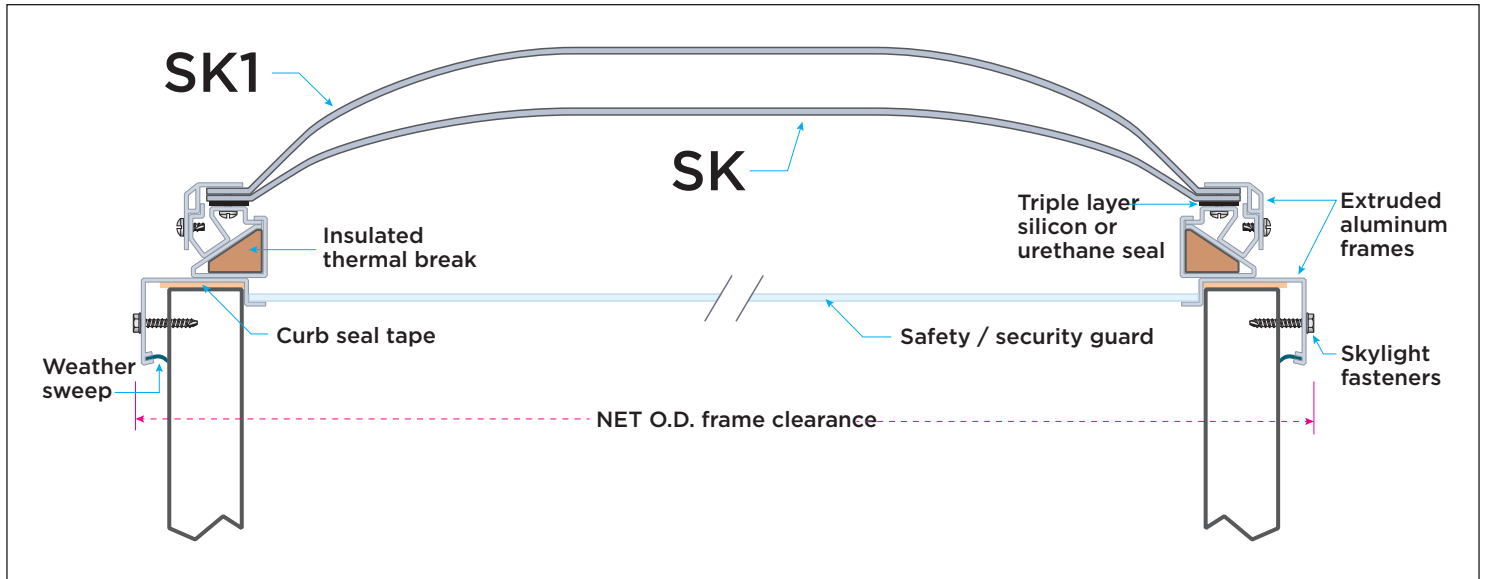
Figure 1: Non-planar skylight
