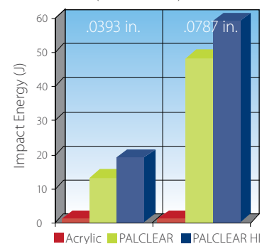
Impact Strength Comparison at 73°F (ISO 6301/1 E50)
