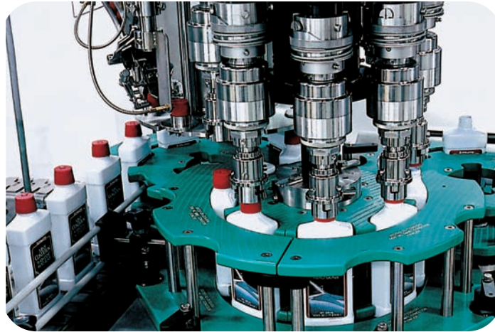
Polystone® M star wheels and guides on filling and capping machinery
