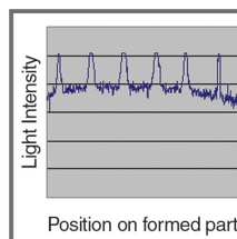
Light intensity across LED light string location
