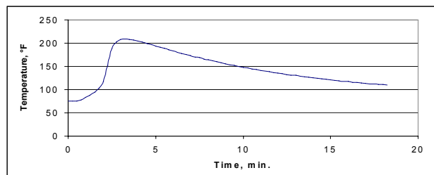
Typical Exotherm Curve for MA420FS in a 10 gm Mass at 74°F (23°C) 5
