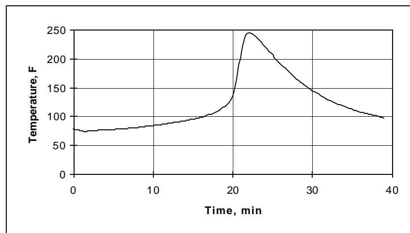
Typical Exotherm Curve for MA310 at 75°F (10 grams) 5
