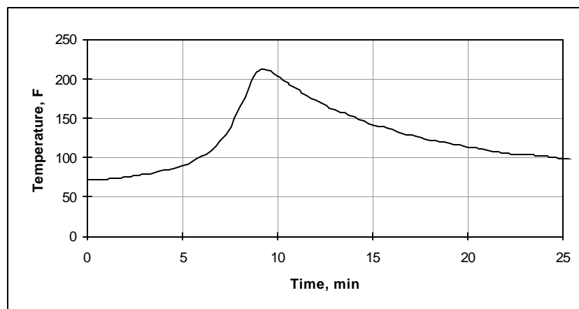
Typical Exotherm Curve for AO420 at 75°F (10 grams) 5
